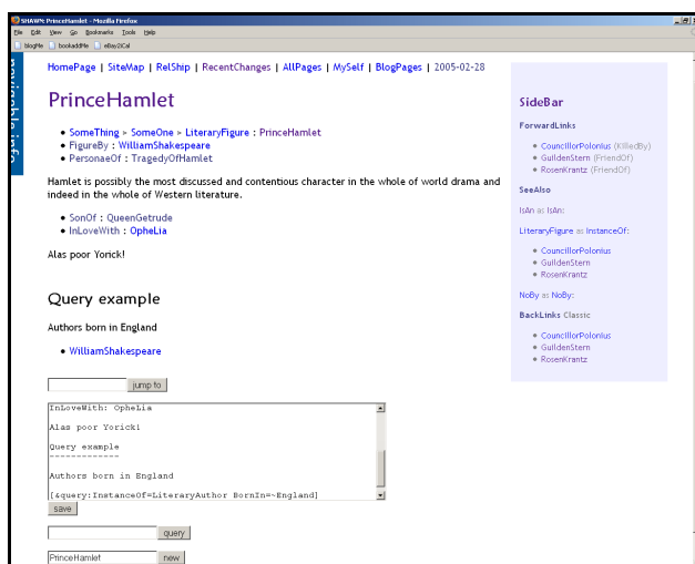
Figure 1. Interface of the SHAWN Wiki prototype.
